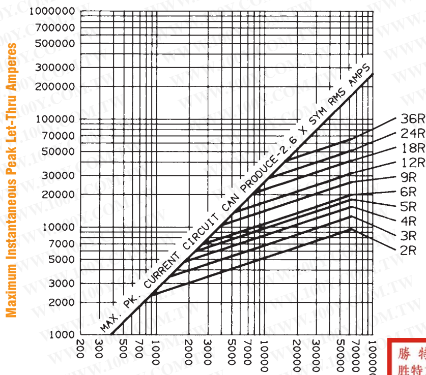
Available Current in RMS Symmetrical Amperes
