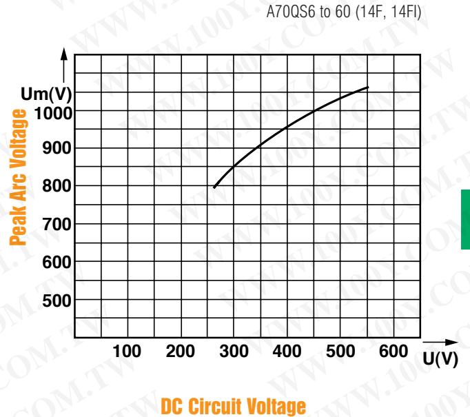
Peak Arc voltage vs. DC circuit voltage
