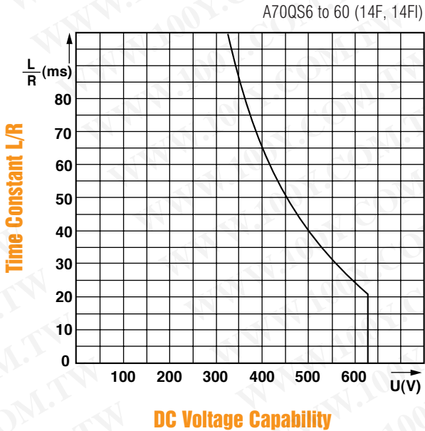
DC Voltage Capabilities vs. Time Constant
