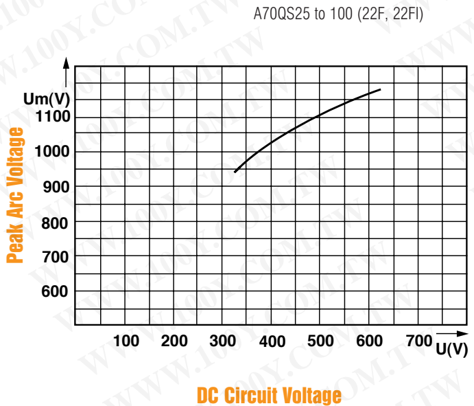
Peak Arc voltage vs. DC circuit voltage
