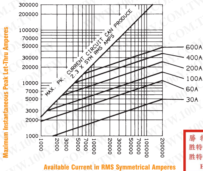
Peak Let-Through Current Data - A6K30 to 600, 600 Volts AC
