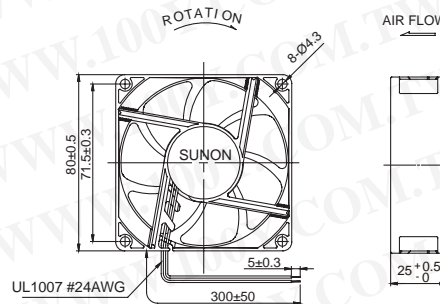
(Units : mm )
