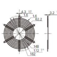
Outlet side
