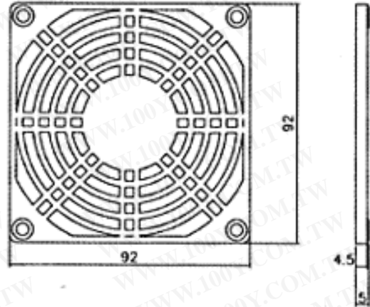
PG-92 FOR 92mm FAN
