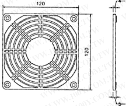
PG-120 BLACK PG-120 WHITE FOR 120mm FAN
