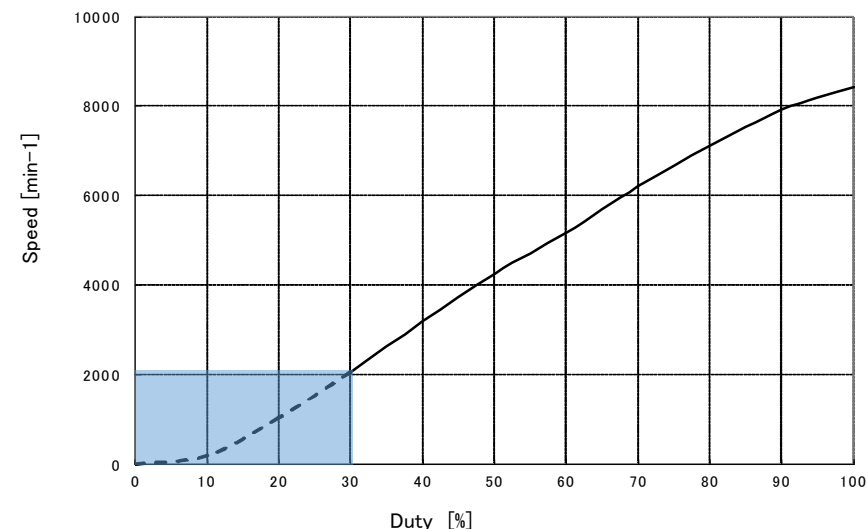
Duty vs Speed Curve <Reference Value> At Rating Voltage, V_{st}(H)=5.0V , f=25kHz , T_a=25^\circ C
