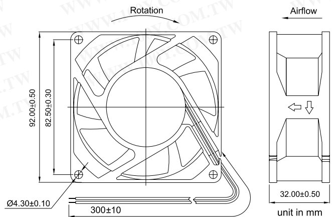
OUTLINE DIMENSIONS
