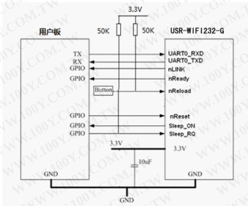
Figure 7. USR-WIFI232-G 硬件连接典型应用
