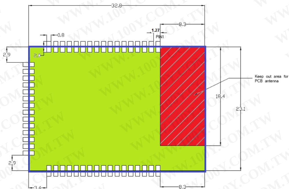
Figure 4. USR-WIFI232-G PCB 元件尺寸
