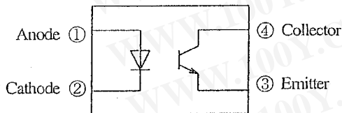
Pin-Number and internal connection diagram
