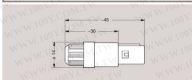
PRG Free socket, key (G) or keys (A, B, C, H and J), with cable collet
