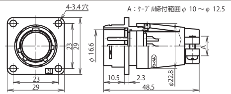
NR-20 ■ -Ad(F)M
