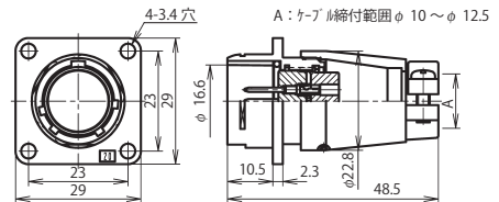
NR-20 ■ -Ad(F)M
