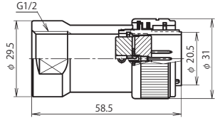
NR-24 ■ -GPM1/2 (注)
