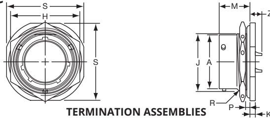
TERMINATION ASSEMBLIES
