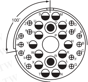
100° Rotation of 36-9 36-18
