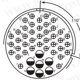
110° Rotation of 36-7 36-17
