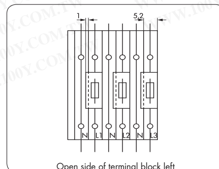
Open side of terminal block left
