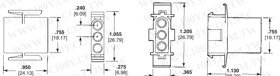
Socket Housing (Plug) Part No. 1-350346-0
