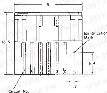
Section X-X
