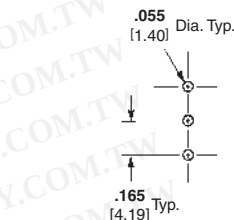
Recommended PC Board Hole Layout
