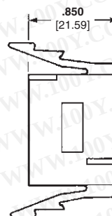
Socket Housing (Plug)
