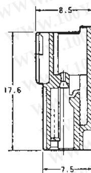
Section X-X
