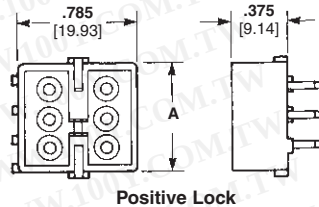
Positive Lock
