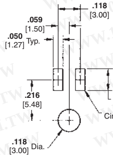
Recommended PC Board Layout * 2 Position
