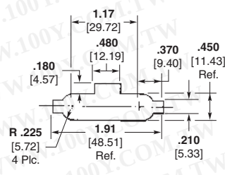
Panel Mount Cutout
