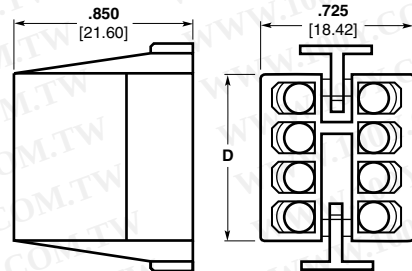
Socket Housing (Plug)
