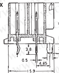
Section X-X
