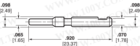
Part Number 794369-1
