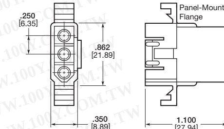
Plug
