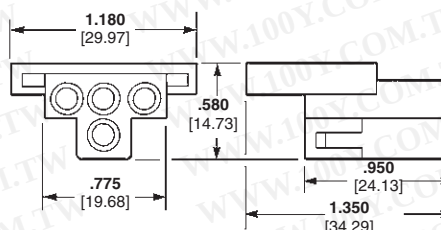
Socket Housing (Plug) Part No. 1-480510-0
