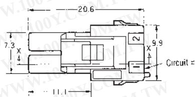
Section X-X
