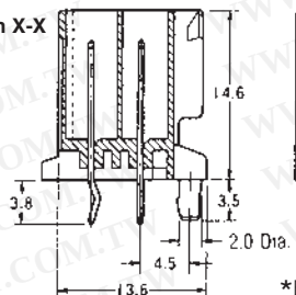
Section X-X
