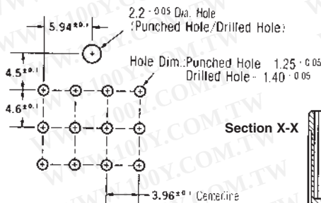
PC Board Layout (Applicable Board Thickness: 1.6 mm)
