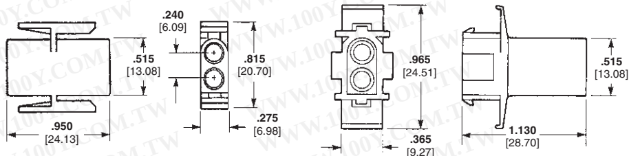
Socket Housing (Plug) Part No. 1-350344-0 Part No. 794699-1 (Black Color High Temp.)
