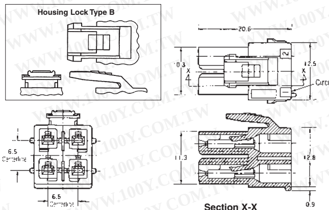
Section X-X
