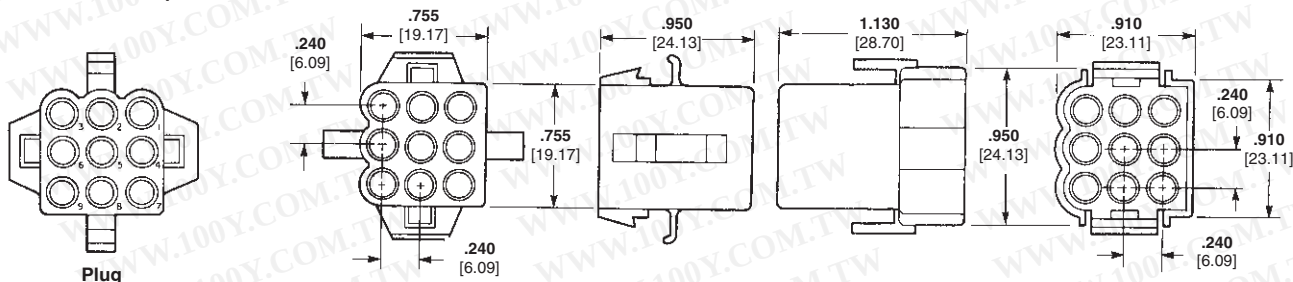
Socket Housing (Plug) Part No. 1-480672-0 Part No. 1586305-1 (Black Color High Temp.)
