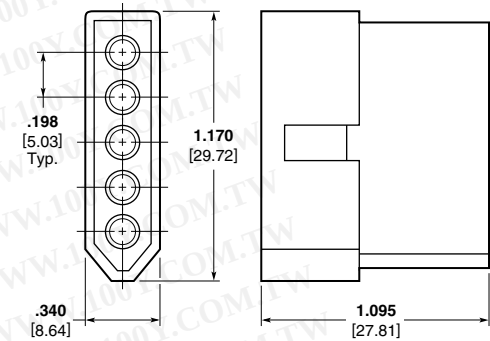
Plug (Free-Hanging)
