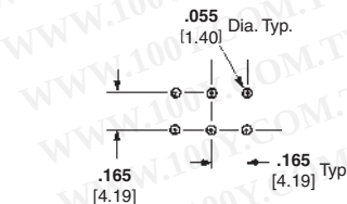
Recommended PC Board Hole Layout
