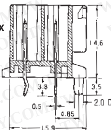
Section X-X
