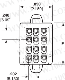
Pin Housing (Cap)
