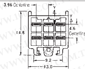
Section Y-Y
