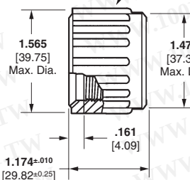
Coupling Ring
