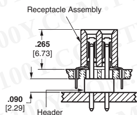
Figure 1 Double-Row, Mod IV, Bottom Entry, Breakaway Header
