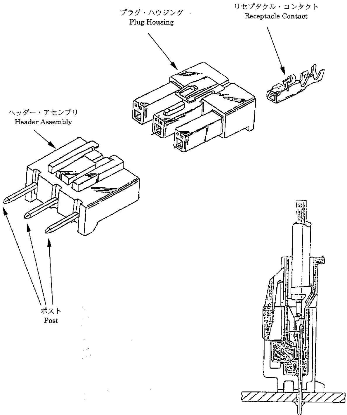
嵌合状態断面図 Cross-sectional View of Mated Connectors
