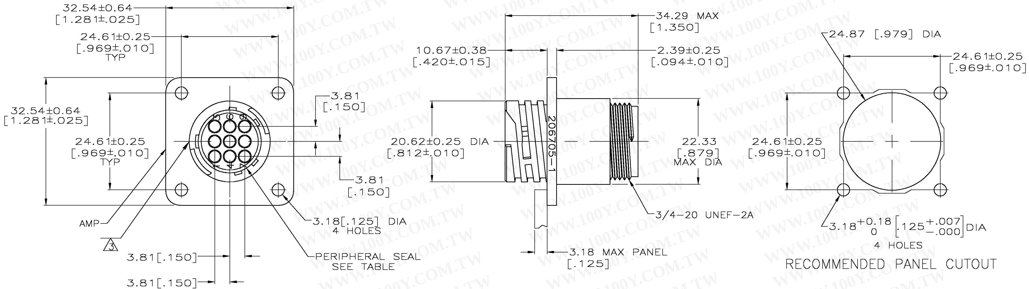
DETAIL A
