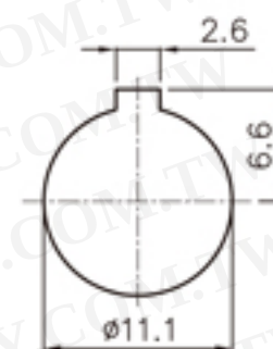
MOUNT HOLE
