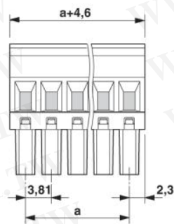
Dimensioned drawing
