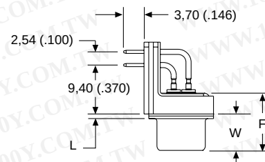
BRACKET, PLASTIC, WITH GROUNDING STRAP
