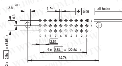
PCB drillhole pattern
