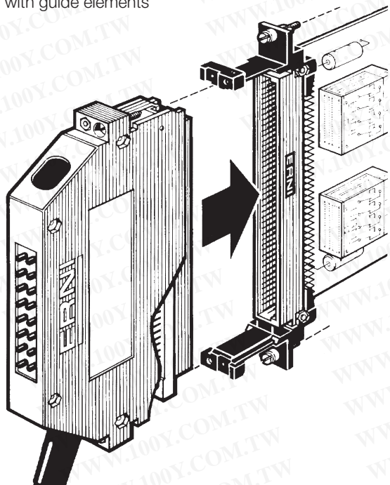
Front panel with guide elements
