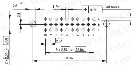
PCB drillhole pattern
