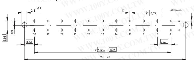
PCB drillhole pattern
