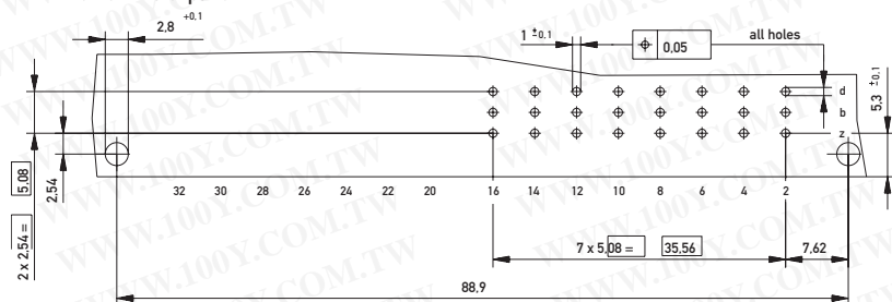
PCB drillhole pattern
