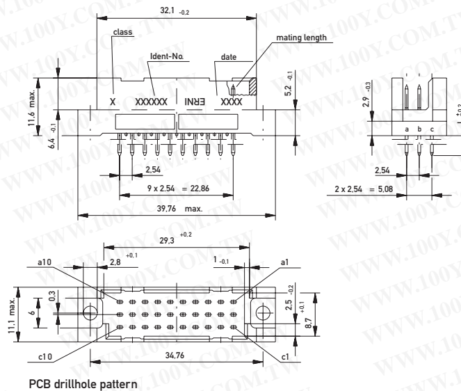
PCB drillhole pattern
