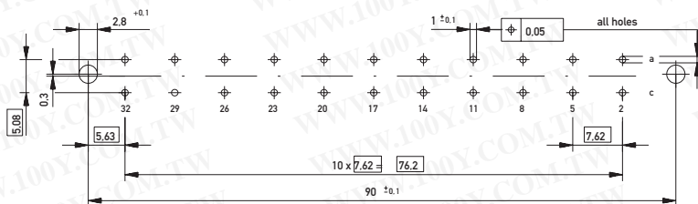
PCB drillhole pattern
