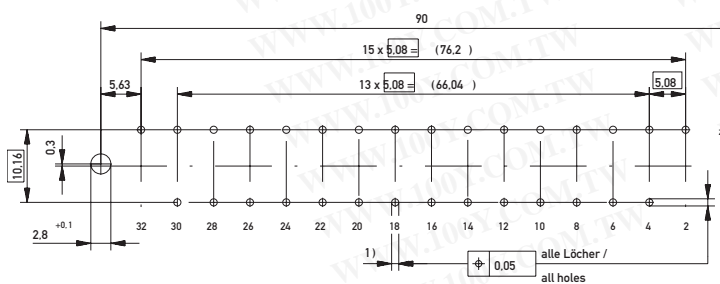
PCB drillhole pattern
