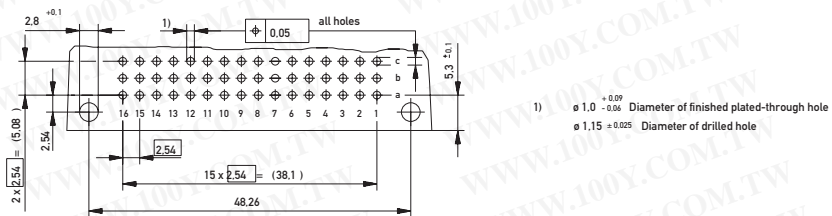
PCB drillhole pattern
