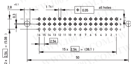
PCB drillhole pattern
