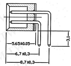
SEC B-B
