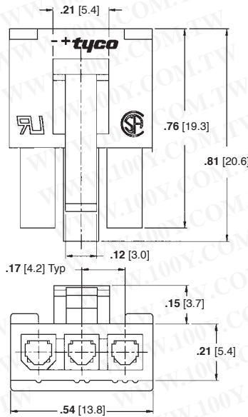
Receptacle Housing
