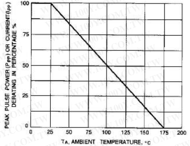
Fig. 2-PULSE DERATING CURVE
