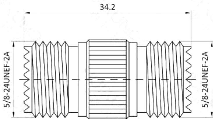
UHF SL16 Female to Female Adapter
