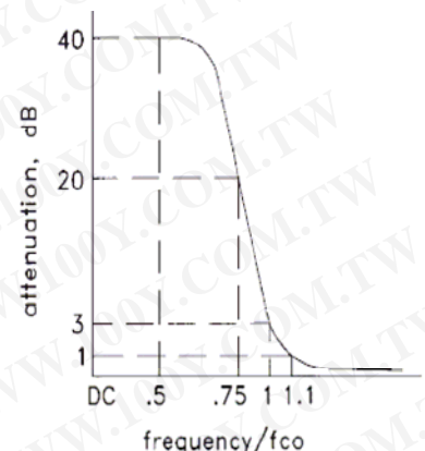
HIGH PASS TYPICAL FREQUENCY RESPONSE
