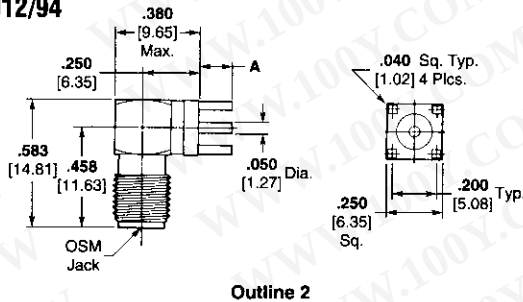
Outline 2
