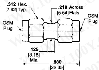
Outline 3
