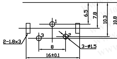
Dimensions of PC board holes(Commend) Bottom View
