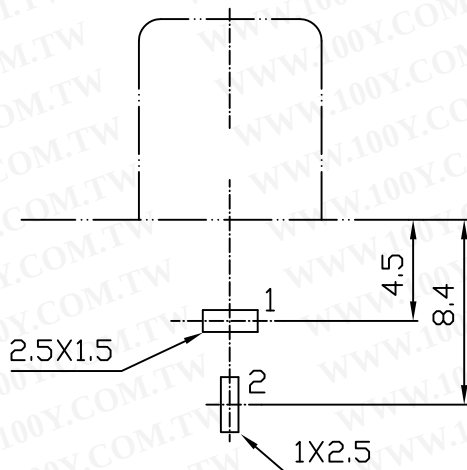
Dimensions of PC board holes(Commend)
