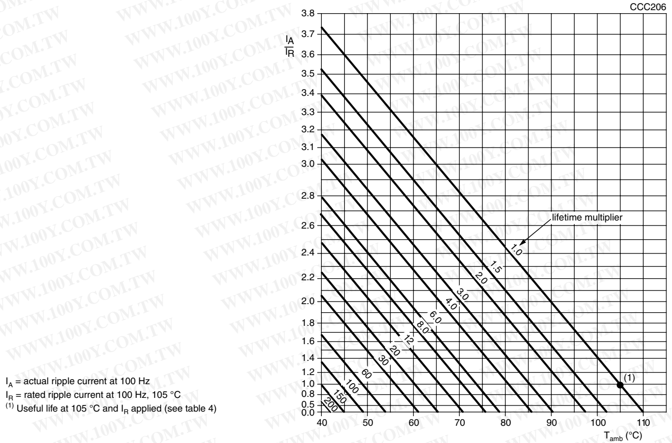
Fig.13 Multiplier of useful life as a function of ambient temperature and ripple current load
