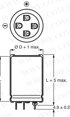
Fig. 5 - Printed wiring pin version (case Ø D = 35 mm)
