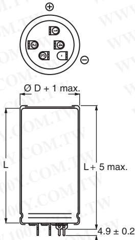
Fig. 7 - Printed wiring pin version (case Ø D = 40 mm)
