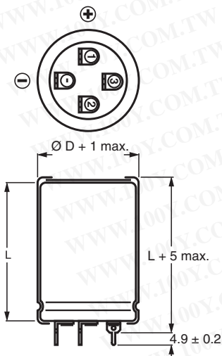
Fig. 3 - Printed wiring pin version (case \varnothing D = 30 mm)
