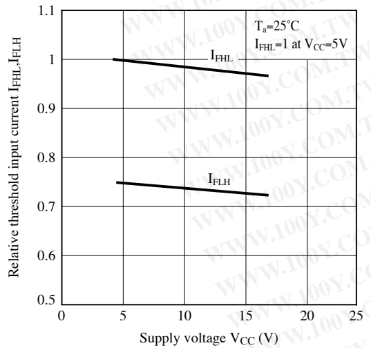
Fig.5 Relative Threshold Input Current vs. Supply Voltage
