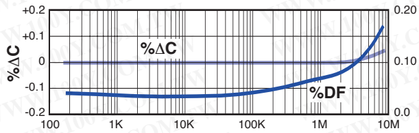
Figure 8. Frequency - Hertz Capacitance & DF vs Frequency - C0G
