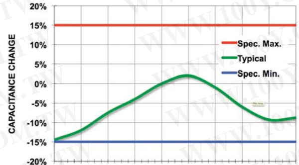
MAXICAP TEMPERATURE COEFFICIENT
