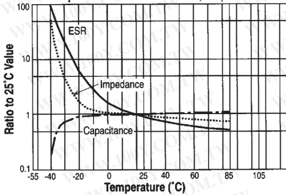
Temperature Characteristics - 98,000 \mu F 10 Vdc
