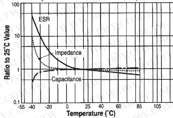
Temperature Characteristics - 29,000 \mu F 50Vdc
