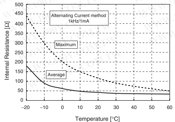
Temperature Characteristics (Internal Resistance (Ri ac))
