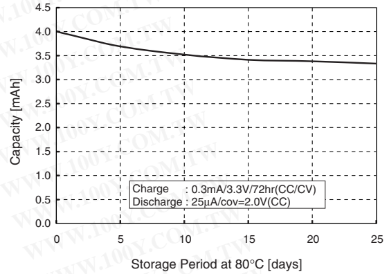
High Temperature Storage Characteristics(80°C)
