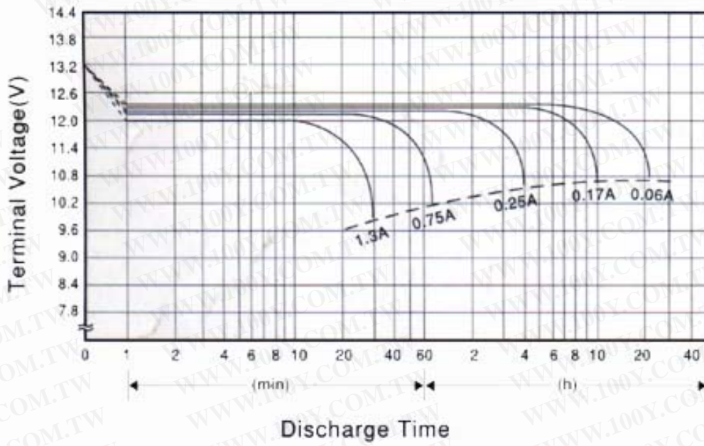
Discharge curves 77°F(25°C)*
