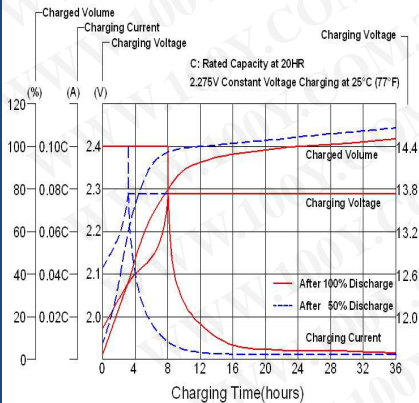
CHARGING CHARACTERISTICS
