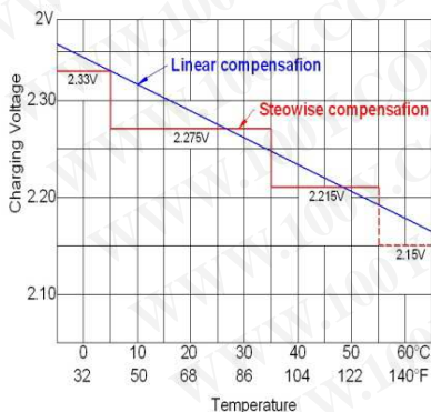
Relationship Between Temperature and Charging Voltage
