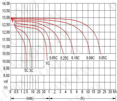
Discharge characteristic at different rates(25°C)
