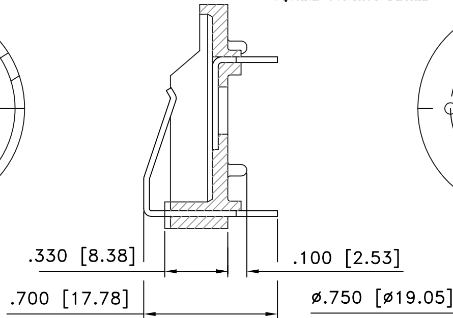
SQUARE CONTACT DETAIL
