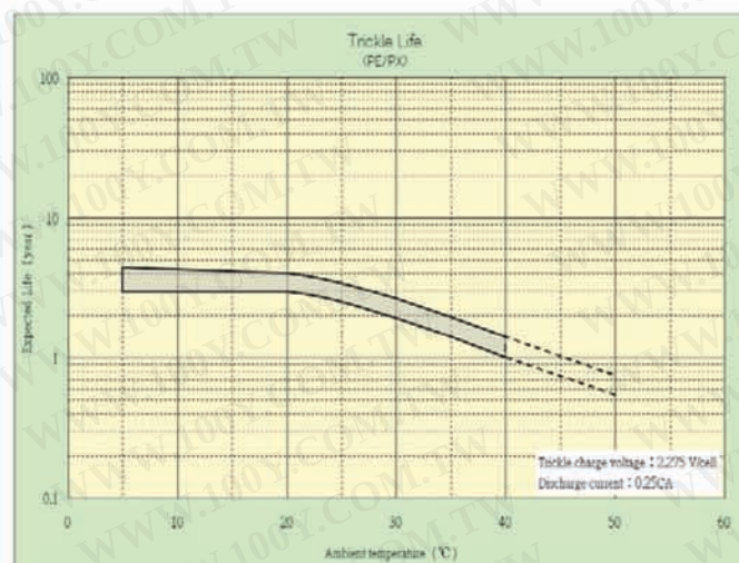
4. 浮充壽命 (Trickle Life)
